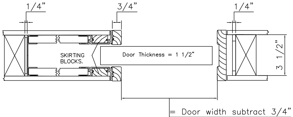
DETAIL SHOWING ARCHTECTURAL UNIT WITH FLAT TIMBER JAMBS
